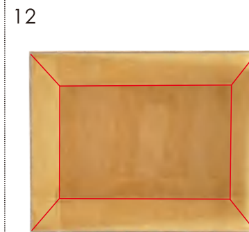
Apply glue to the glass joint and scrape lightly for penetration (red line indicates the joint).
