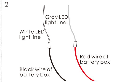
2 Connect the Black and LED white wires of the battery box, as well as the red and gray LED gray wires of the battery box, respectively
