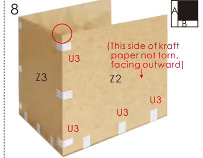
The junction of two pieces of plexiglass needs to be fixed with U3 (to prevent the plexiglass falling off)
